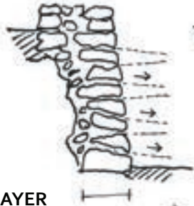
1) WALL IS TOO THIN, STONES LEAN OUTWARDS
