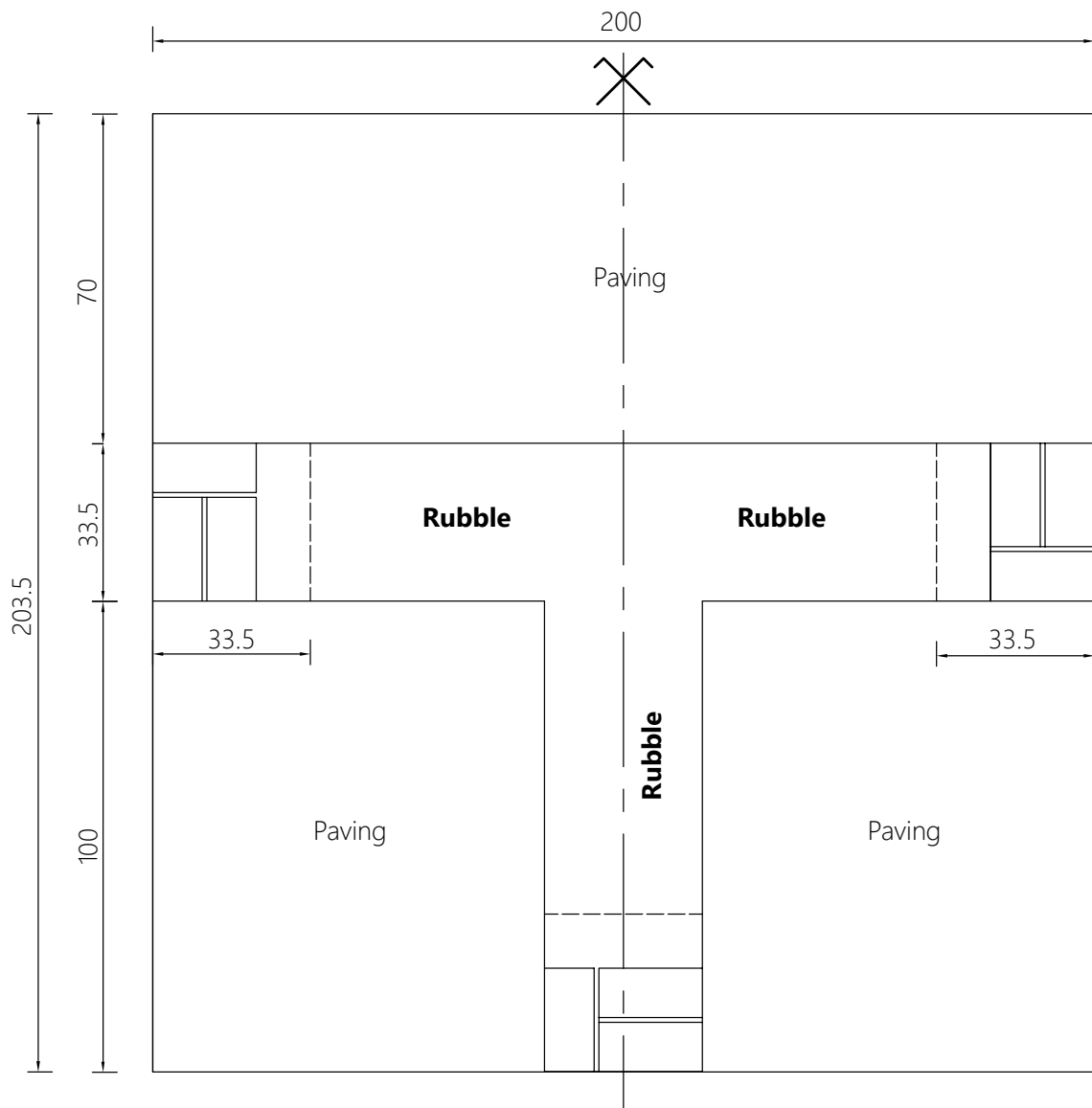
Top view • Scale : 1/15
